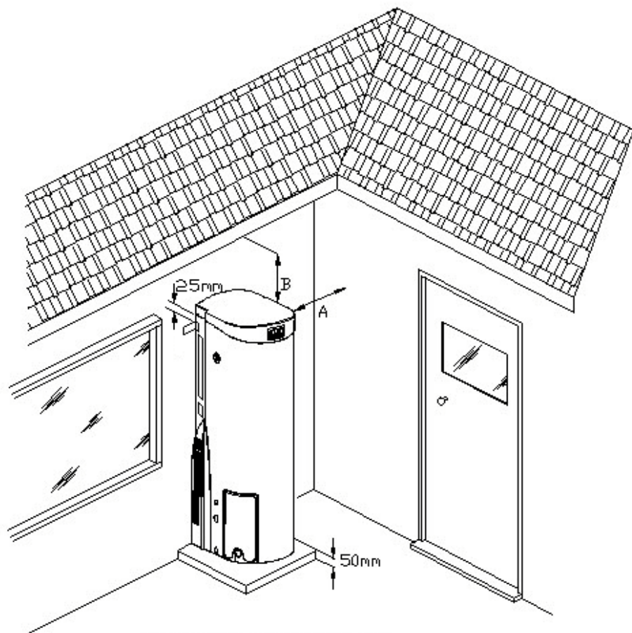
Figure 1: Clearances Required for Outdoor Installation
