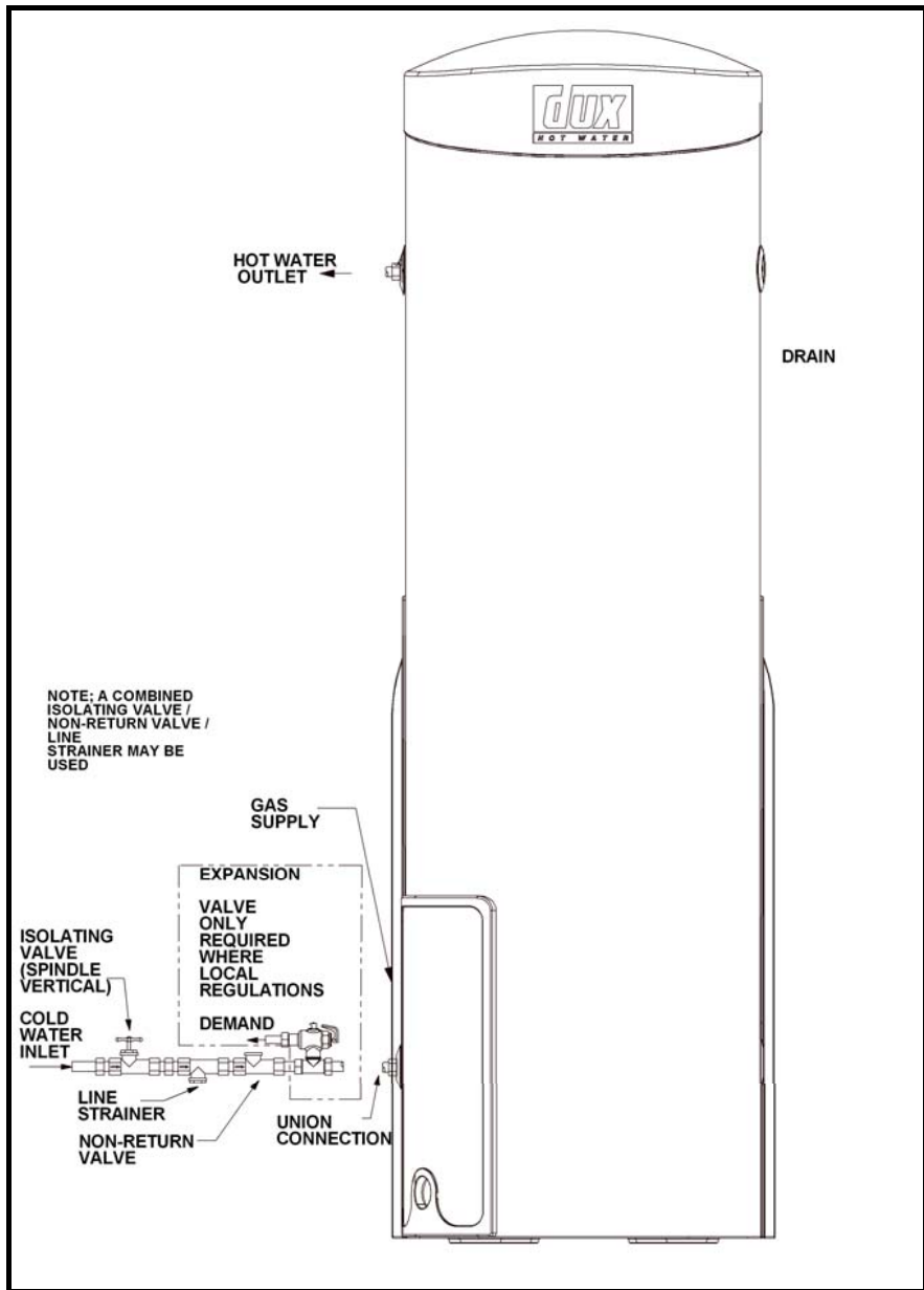
Figure 2: Hot & Cold Water Connections
