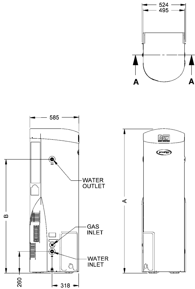
Figure 5: Dimensions of Unit
